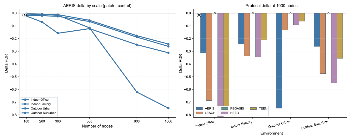
Figure 4. S11 matched patch-control evidence. (a) AERIS delta trajectories over node counts (patch - control). (b) Protocol deltas at 1000 nodes across environments. Negative deltas indicate lower PDR under patch mode.
