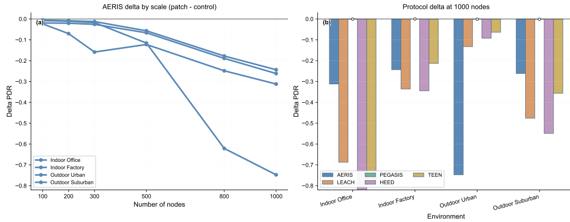
Figure 5. S11 matched patch-control evidence. (a) AERIS delta trajectories over node counts (patch - control). (b) Protocol deltas at 1000 nodes across environments. Negative deltas indicate lower PDR under patch mode.
