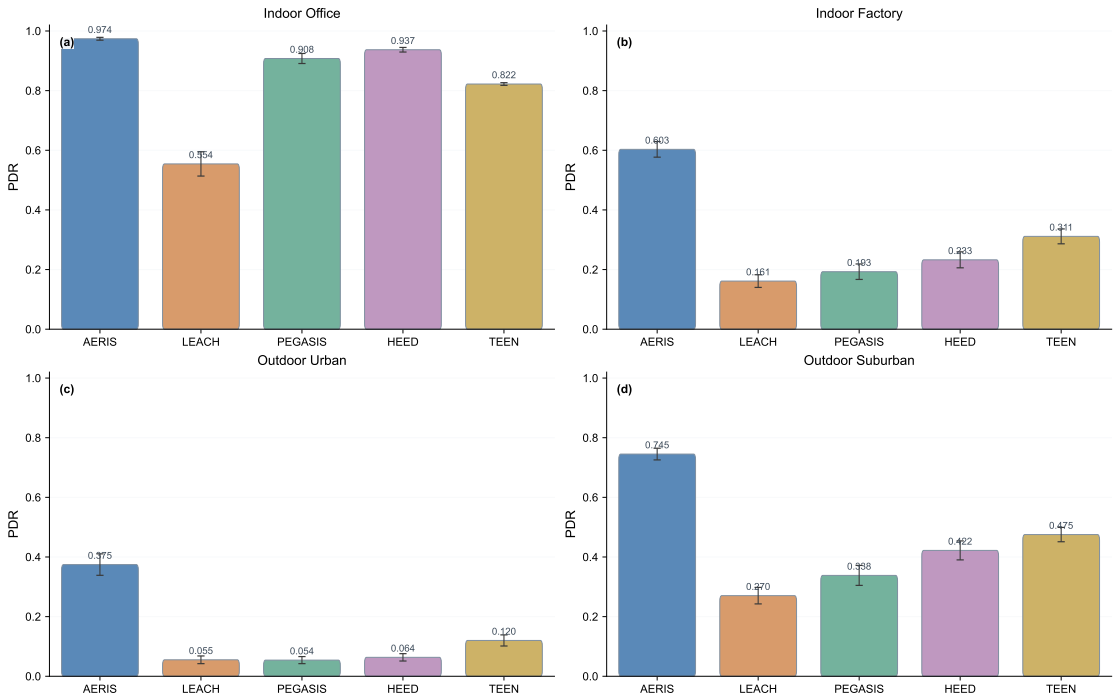
Figure 1. PDR comparison panel at 100 nodes (4 environments, n=30).
