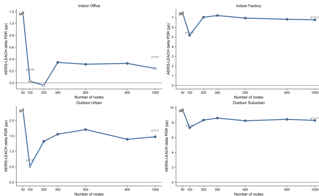
Figure 7. NS-3 trend panel over 50–1000 nodes (AERIS–LEACH delta in percentage points). Hollow markers denote non-significant cells after Holm correction.
