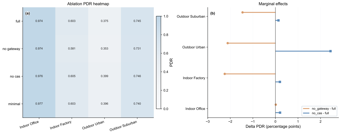
Figure 2. Ablation panel: heatmap and marginal effects (n=30).
