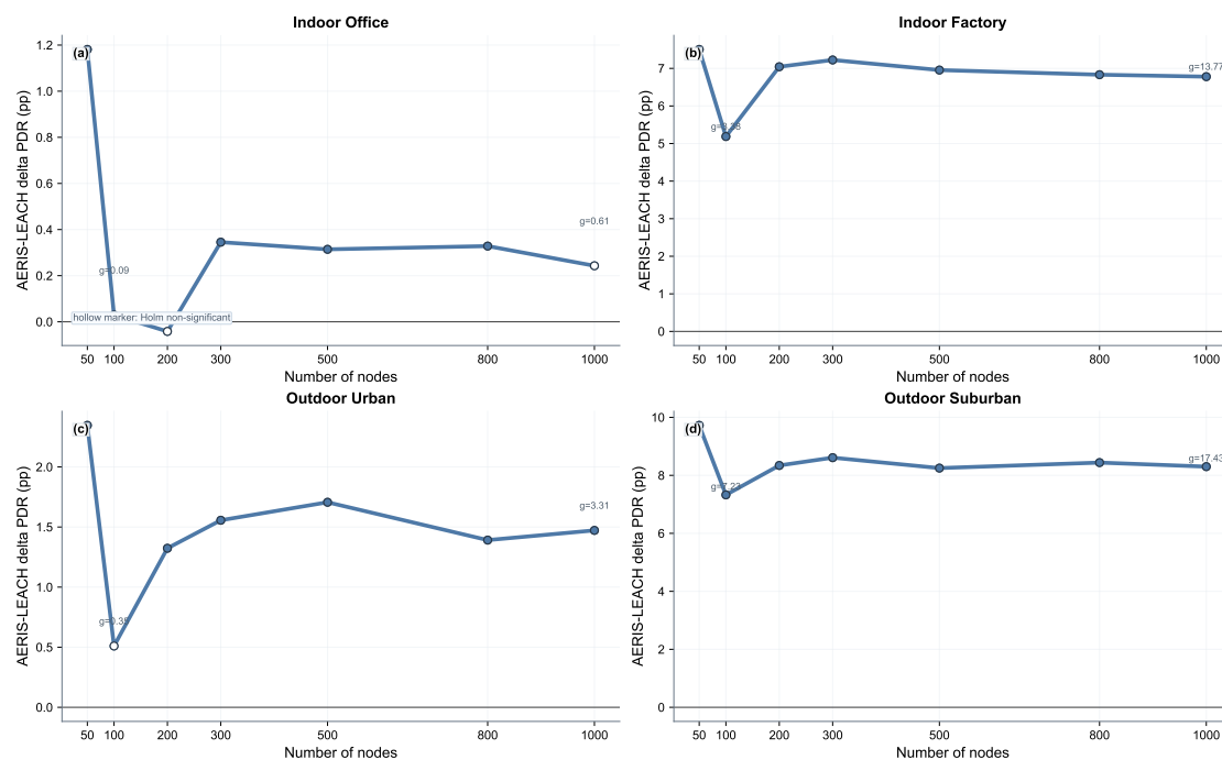
Figure 11. NS-3 trend panel over 50–1000 nodes (AERIS–LEACH delta in percentage points). Hollow markers denote non-significant cells after Holm correction.
