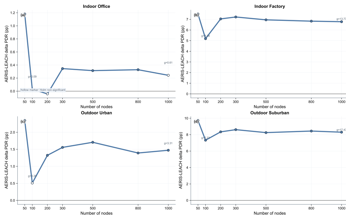
Figure 12. NS-3 trend panel over 50–1000 nodes (AERIS–LEACH delta in percentage points). Hollow markers denote non-significant cells after Holm correction.
