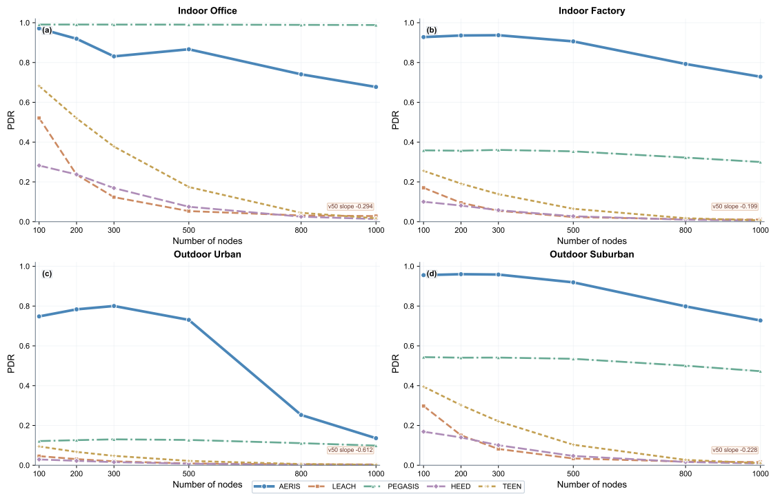
Figure 4. v50-rigor scalability trends over node counts (balanced n=3200 per environment-node-protocol cell) with 95% CI bands. Explicit collision and relay modeling are enabled. AERIS remains rank-1 in three environments and declines with scale in all four environments.
