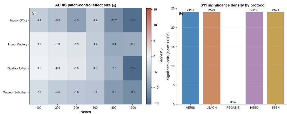
Figure 10. S11 significance density and effect-size map. Panel (a) reports AERIS Hedges' g by environment and node count for patch-control differences. Panel (b) reports the number of Holm-significant cells per protocol (out of 24).
