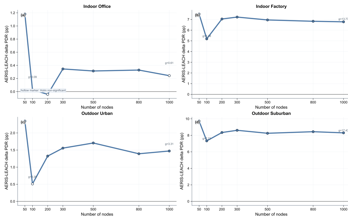
Figure 12. NS-3 trend panel over 50–1000 nodes (AERIS–LEACH delta in percentage points). Hollow markers denote non-significant cells after Holm correction.
