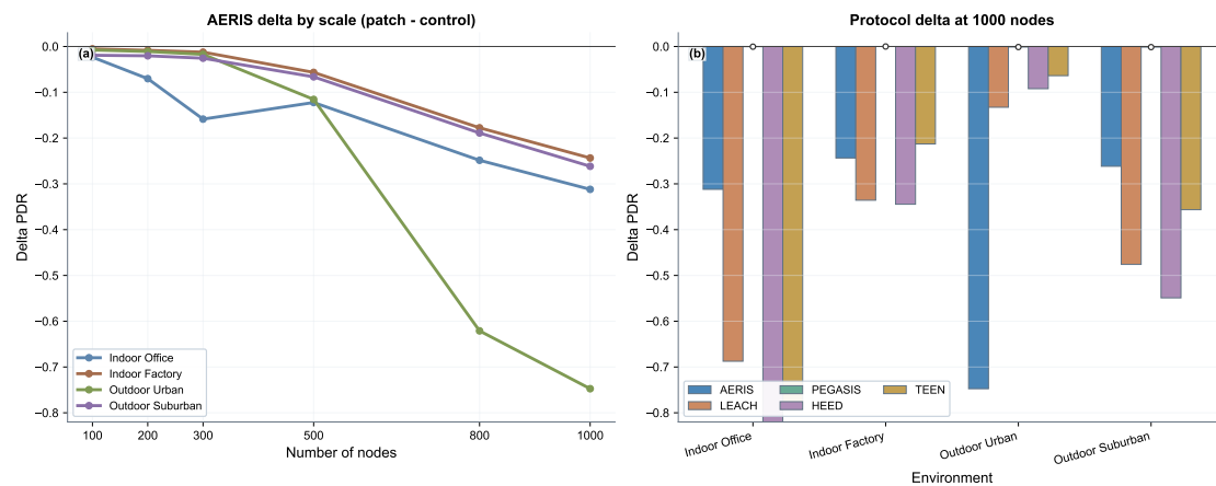
Figure 9. S11 matched patch-control evidence. (a) AERIS delta trajectories over node counts (patch - control). (b) Protocol deltas at 1000 nodes across environments. Negative deltas indicate lower PDR under patch mode.
