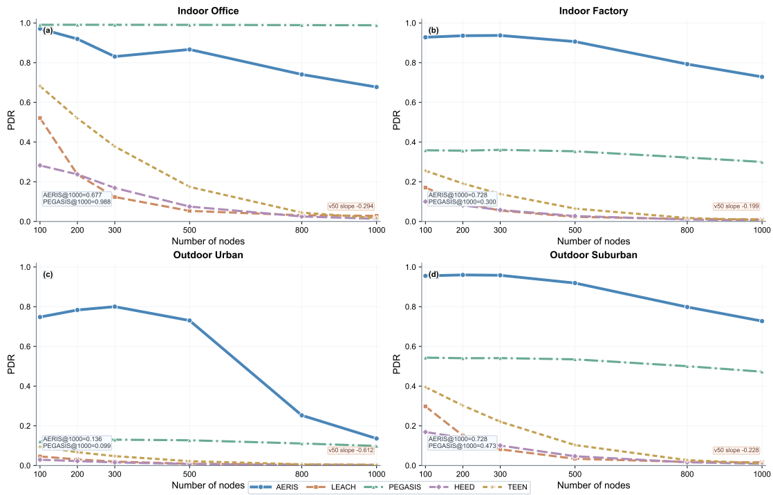
Figure 4. Primary large-scale scalability trends over node counts (balanced n=3200 per environment-node-protocol cell) with 95% CI bands. Explicit collision and relay modeling are enabled. AERIS remains rank-1 in three environments and declines with scale in all four environments.
