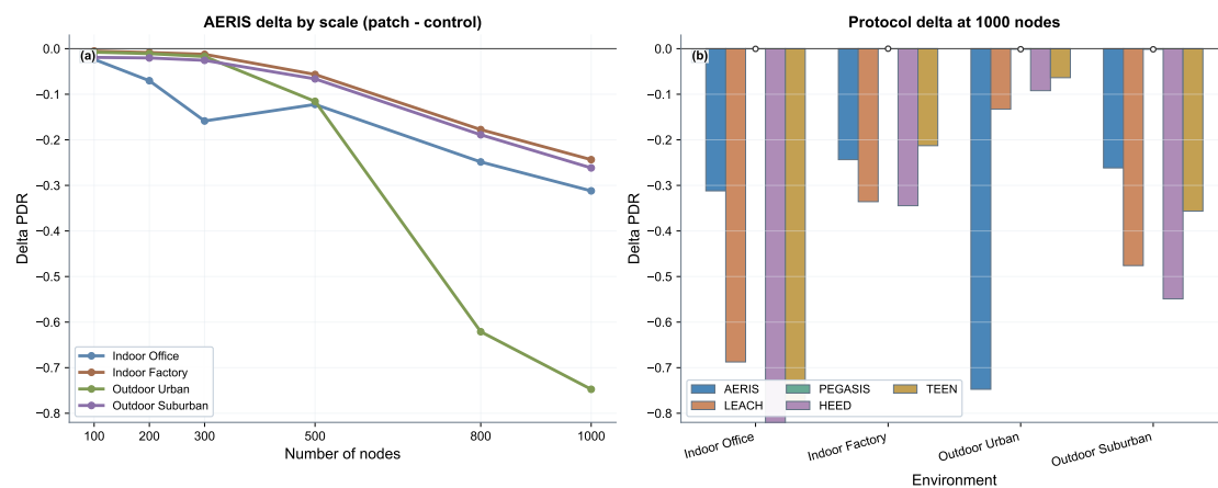
Figure 6. Matched patch-control evidence. (a) AERIS delta trajectories over node counts (patch - control). (b) Protocol deltas at 1000 nodes across environments. Negative deltas indicate lower PDR under patch mode.
