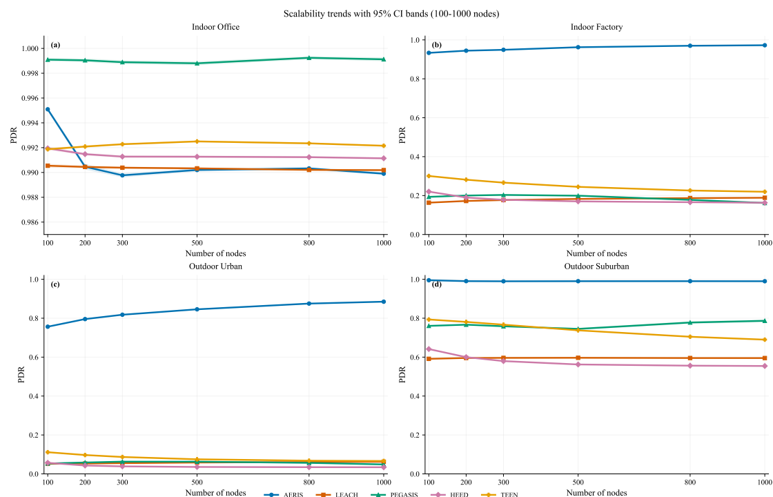
Figure 3. Scalability trends over node counts (indoor_factory n=650 , other environments n=550 ) with 95% CI bands.
