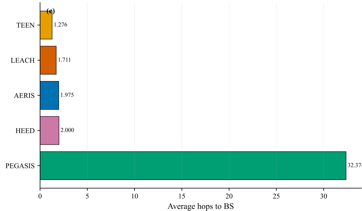
Hop-latency ranking
