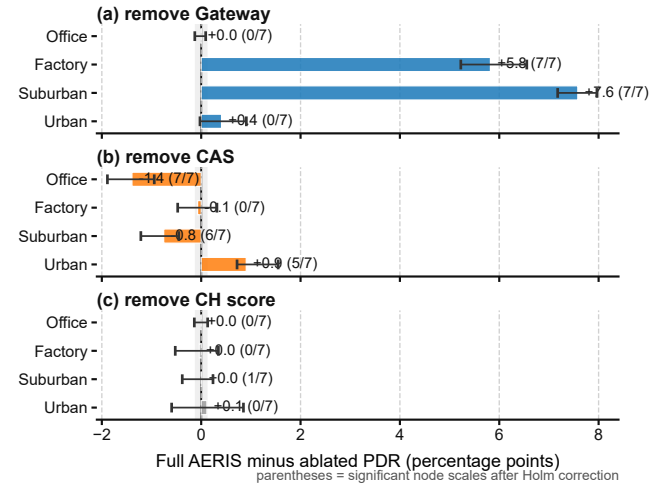
Fig. 4. Expanded NS-3 AERIS ablation across four environments and 50–1000 nodes ( n = 30 per cell). Bars report the mean full-minus-ablated PDR contribution over the seven node scales; intervals show the observed cell range, and parentheses give the number of significant node-scale cells after Welch tests with Holm correction.
