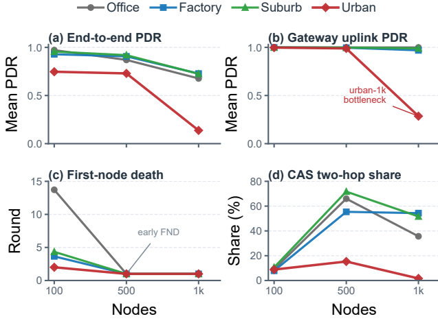
Fig. 5. AERIS mechanism study from 400 replicates per environment-node cell across 12 cells (4800 runs total). The four panels track end-to-end PDR, Gateway-uplink PDR, first-node death (FND), and CAS two-hop share over node scale.
