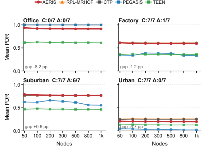
C/A = AERIS rank-1 cells against classical/all baselines; gap = mean AERIS minus best non-AERIS.
