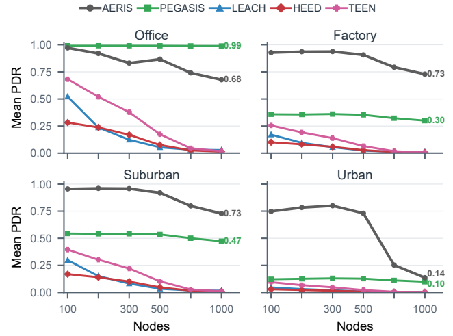
Fig. 3. Stress layer. Collision-aware adapted Python stress test across four environments and 100–1000 nodes ( n = 3200 per cell). LEACH, HEED, and TEEN are minimally relay-enabled; this layer tests collision-and-relay stress and is not canonical ranking evidence.
