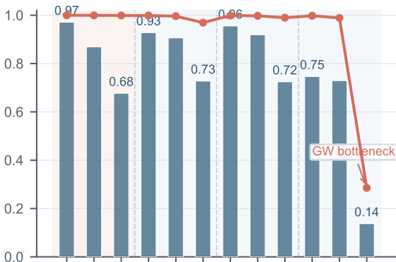
PDR / GW
