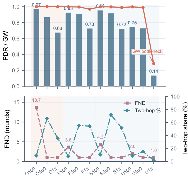
Fig. 5. Corrected 400-replicate AERIS mechanism matrix across the audited 12 environment-node cells. The top panel shows end-to-end PDR together with gateway uplink PDR; the lower panel shows first-node death and the share of CAS two-hop decisions. Gateway remains near-perfect in office, factory, and suburban cells, but collapses at urban-1000.
