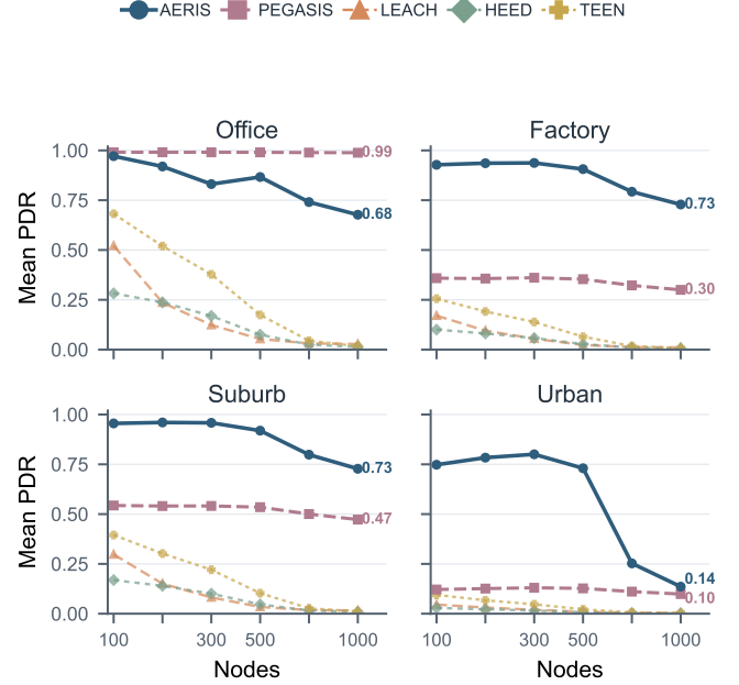
Fig. 3. Strict-physics Python adapted stress test across four environments and 100–1000 nodes ( n = 3200 per cell). LEACH, HEED, and TEEN appear here in minimally relay-enabled form for strict-layer comparability; this layer is used as stress evidence, not as the sole fairness anchor.
