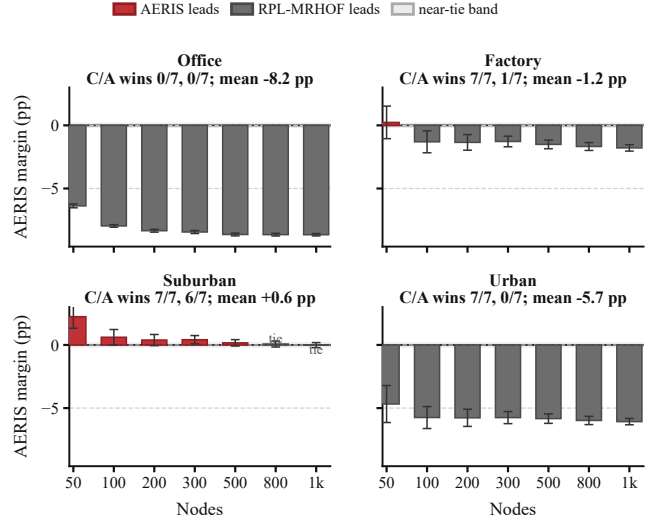
Fig. 2. Expanded NS-3 boundary sweep across four environments and 50–1000 nodes ( n = 30 per cell). Each bar reports mean PDR(AERIS) minus the strongest non-AERIS baseline in percentage points; whiskers show approximate 95% confidence intervals for the gap. Positive bars favor AERIS, negative bars favor the strongest boundary baseline, and the gray band marks the \pm 0.1 percentage-point near-tie region. The title reports AERIS rank-1 coverage against classical/all baselines (C/A).
