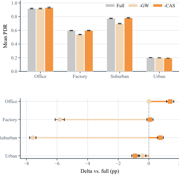
Fig. 4. Expanded NS-3 AERIS ablation across four environments and 50–1000 nodes ( n = 30 per cell). Top: mean PDR of full AERIS, no-Gateway, and no-CAS variants. Bottom: ablated-minus-full PDR delta in percentage points; negative values indicate that the removed module improves delivery in the full protocol. Whiskers show approximate 95% confidence intervals over the seven node-scale means.
