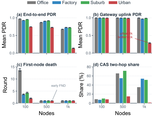
Fig. 5. AERIS mechanism study from 400 replicates per environment-node cell across 12 cells (4800 runs total). The four panels use grouped bars to show end-to-end PDR, Gateway-uplink PDR, first-node death (FND), and CAS two-hop share by environment and node scale.
