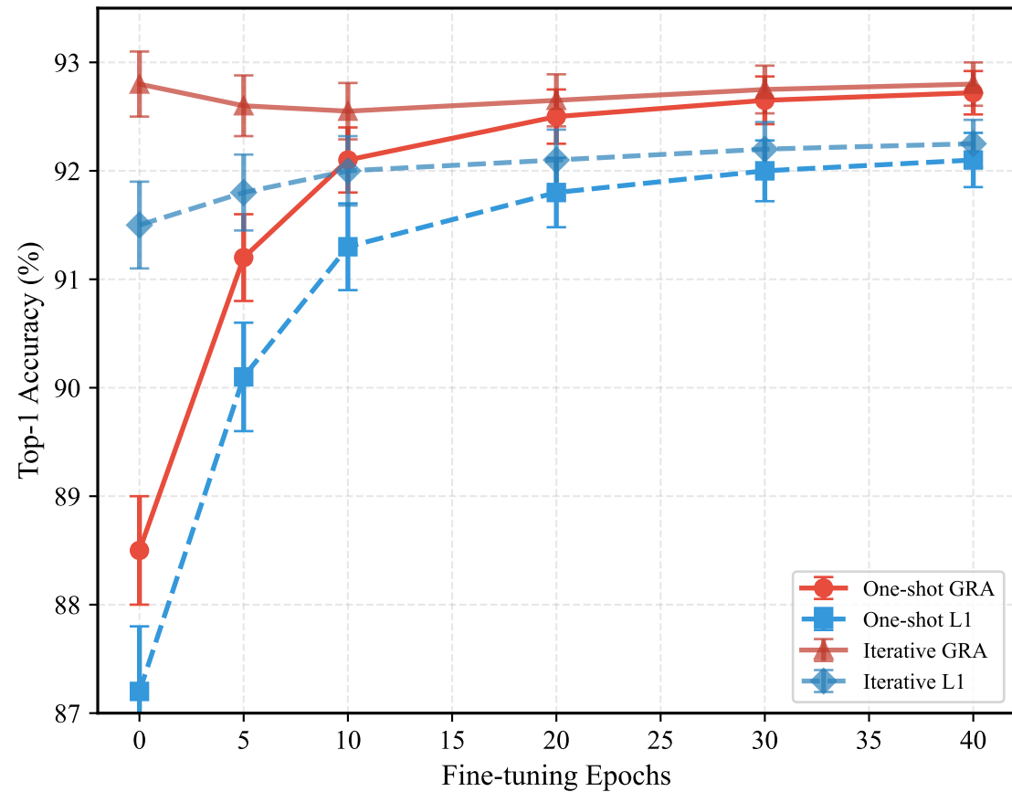
(a) Convergence: One-shot vs Iterative (50% pruning)
