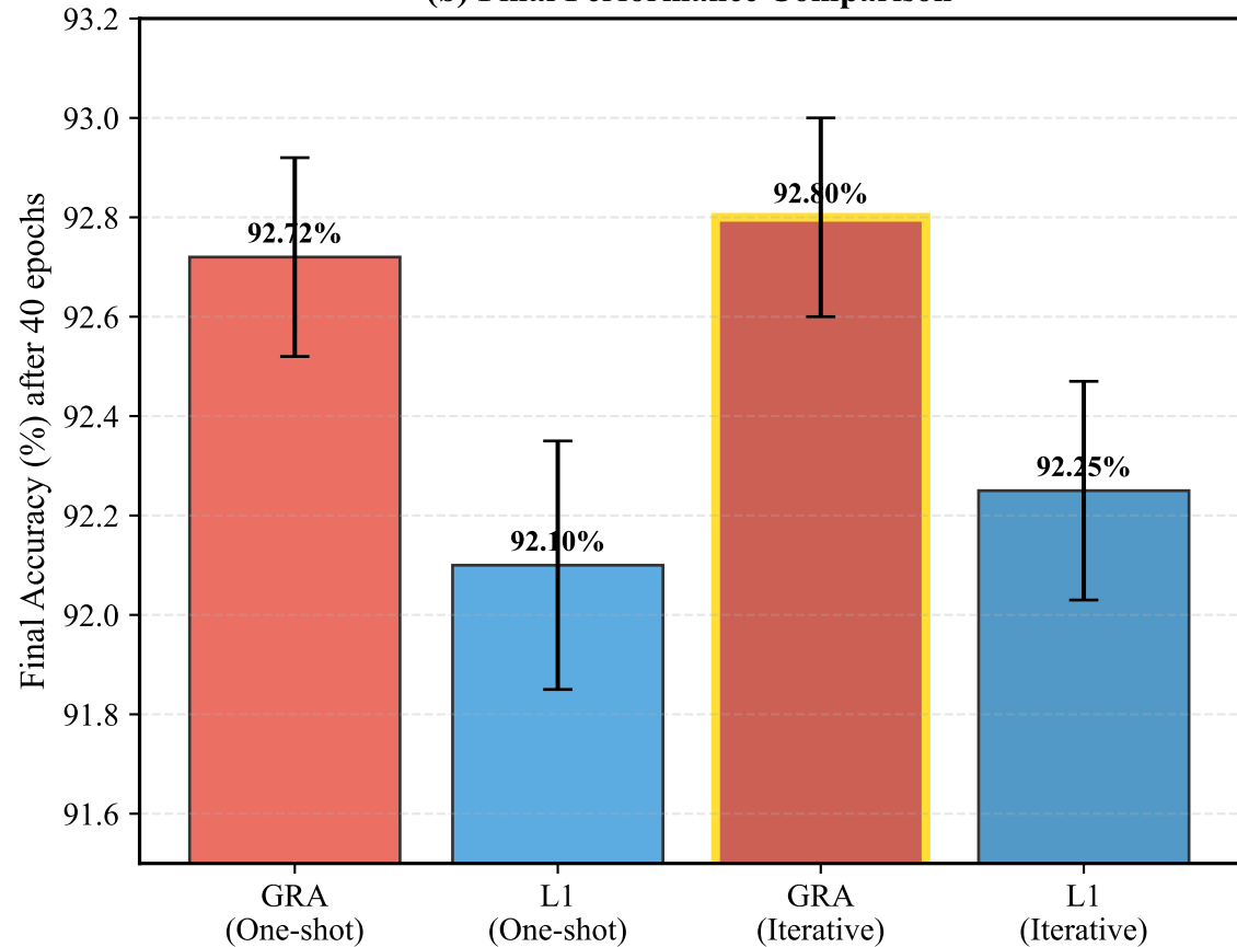
(b) Final Performance Comparison
