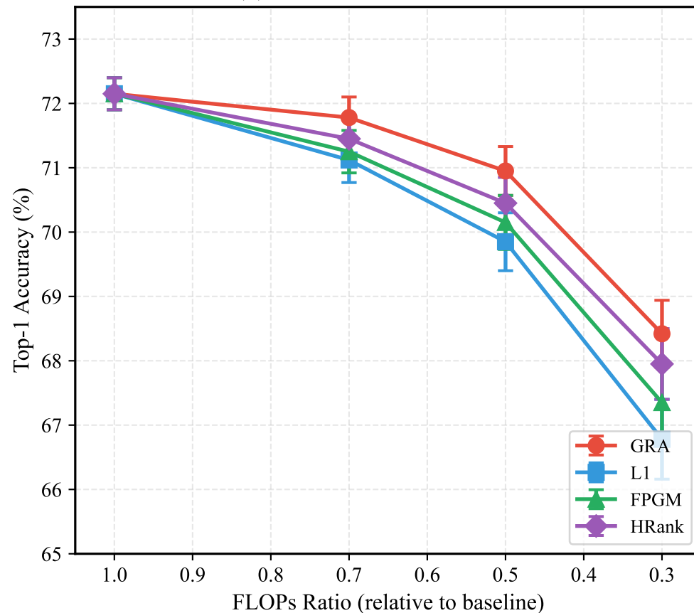
(b) ResNet-56 on CIFAR-100
