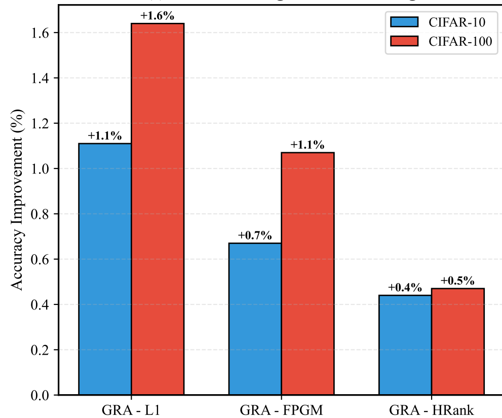
(c) GRA Advantage at 70% Pruning
