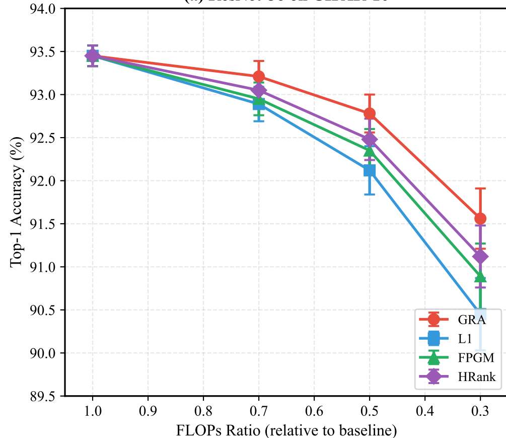
(a) ResNet-56 on CIFAR-10
