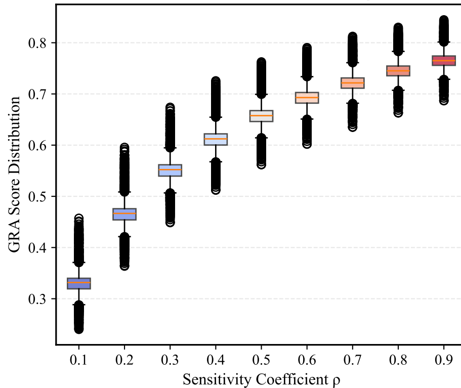
(b) Score Distribution across \rho
