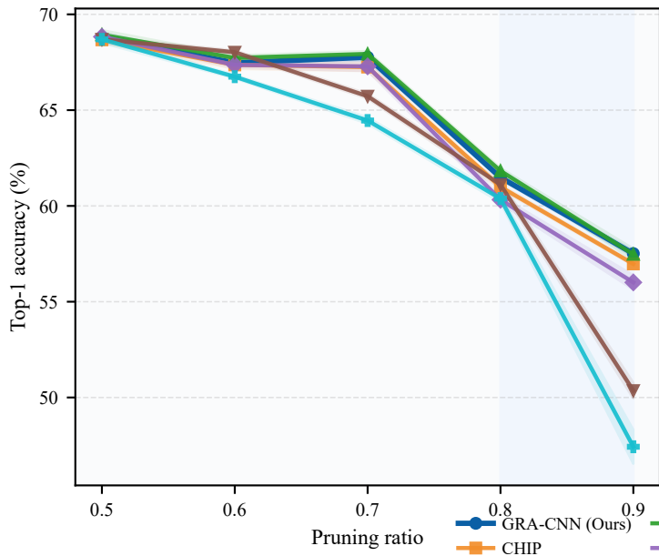
ResNet-56 / CIFAR-100
