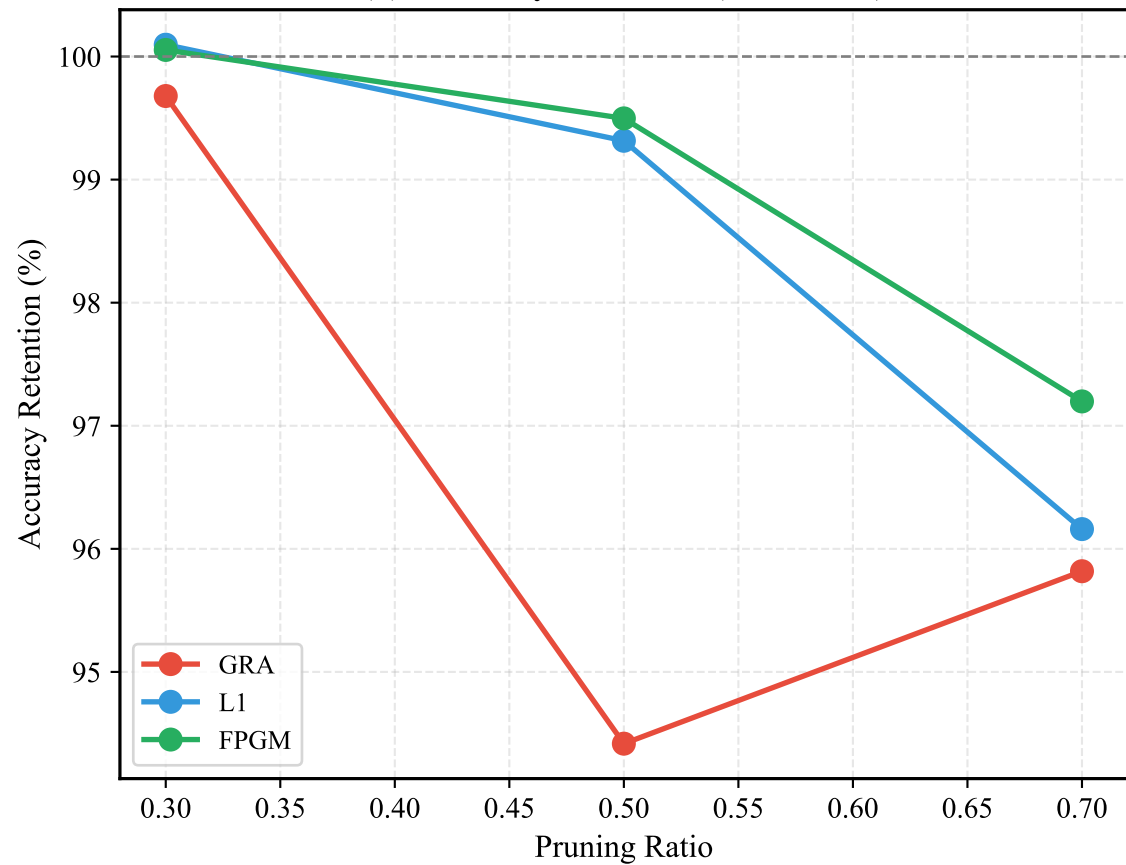
(b) Accuracy Retention (ResNet-56)
