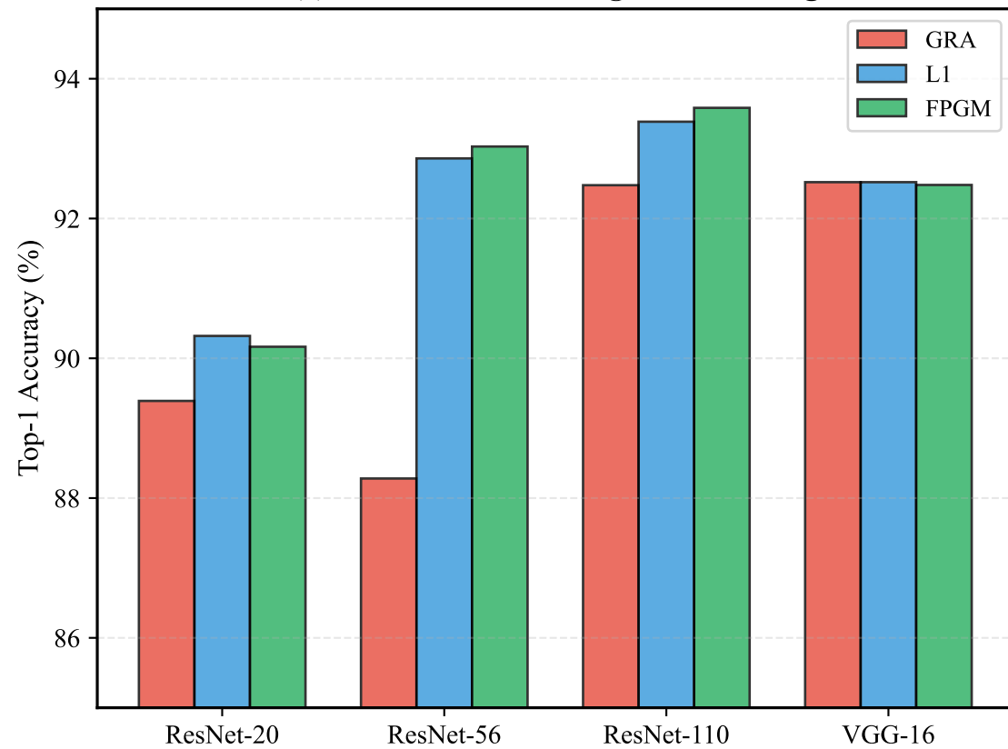
(a) Cross-Architecture @ 50% Pruning
