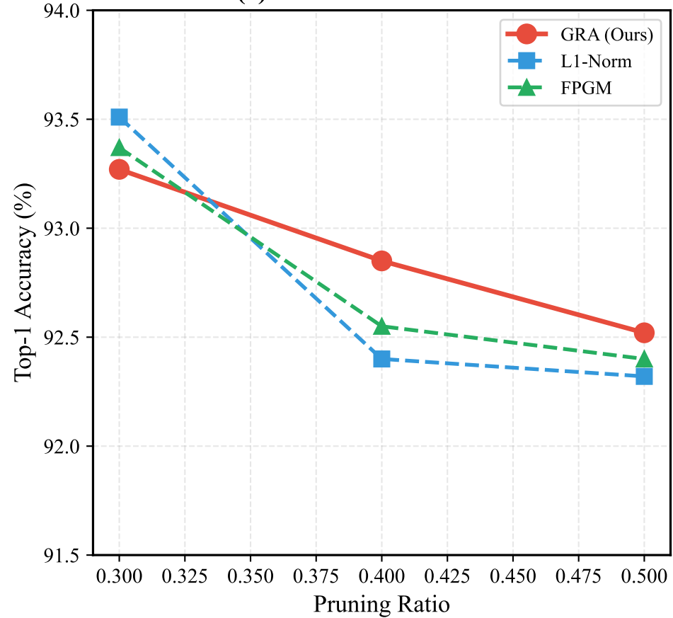
(a) ResNet-56 / CIFAR-10
