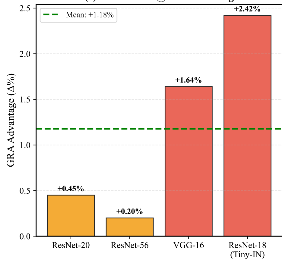
(c) GRA vs L1 @ 50% Pruning
