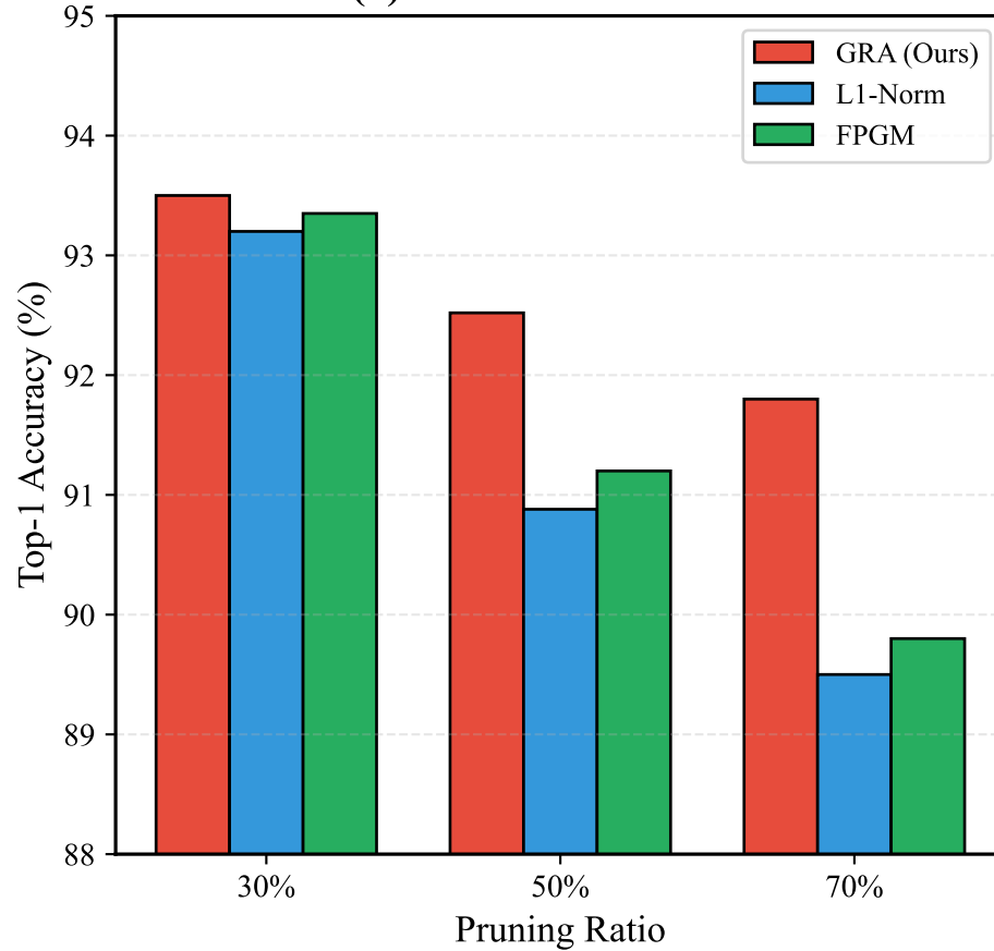
(b) VGG-16 / CIFAR-10
