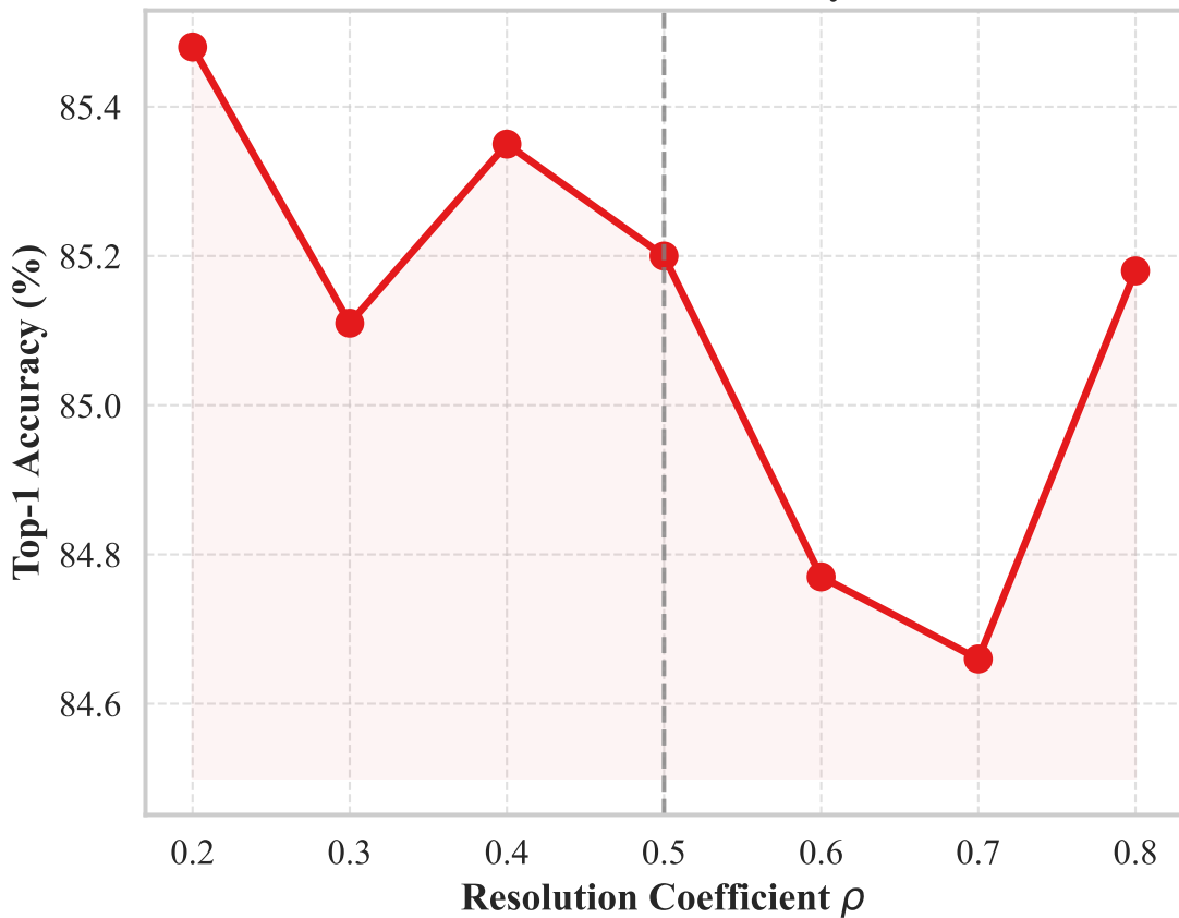
ResNet-20 Sensitivity
