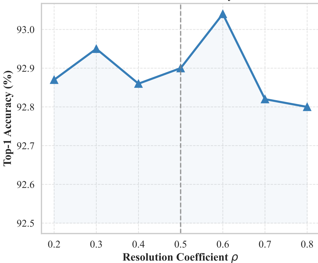
ResNet-56 Sensitivity
