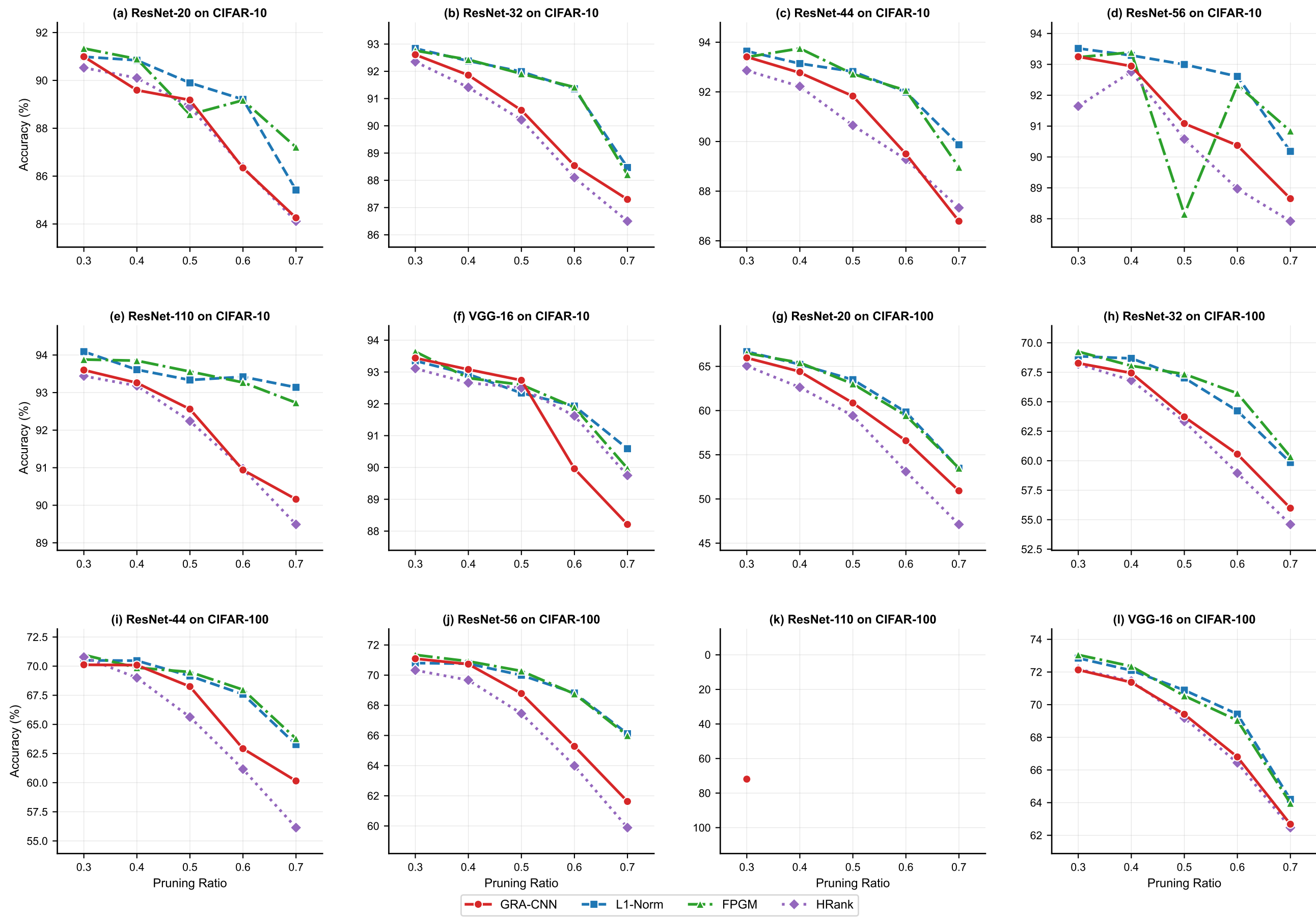
Figure 2: Pruning Performance Across Architectures and Datasets
