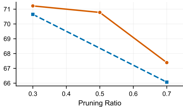
(b) ResNet-56
