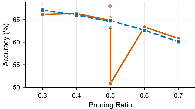
(a) ResNet-20
