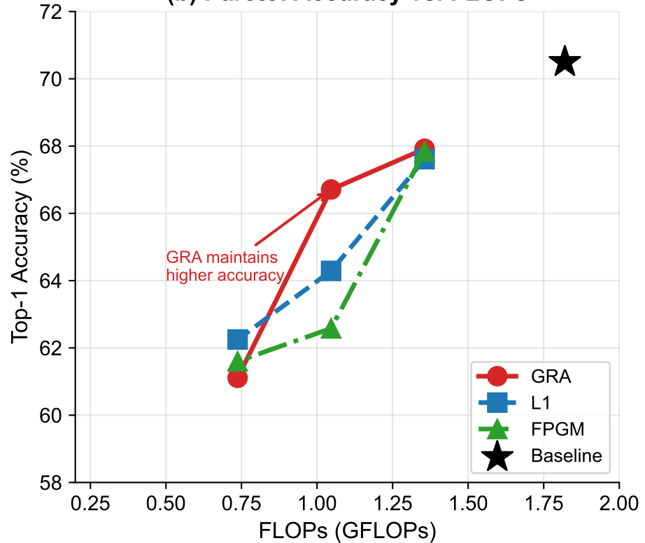
(b) Pareto: Accuracy vs. FLOPs
