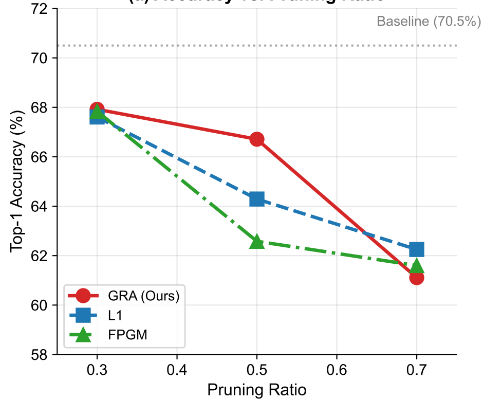
(a) Accuracy vs. Pruning Ratio
