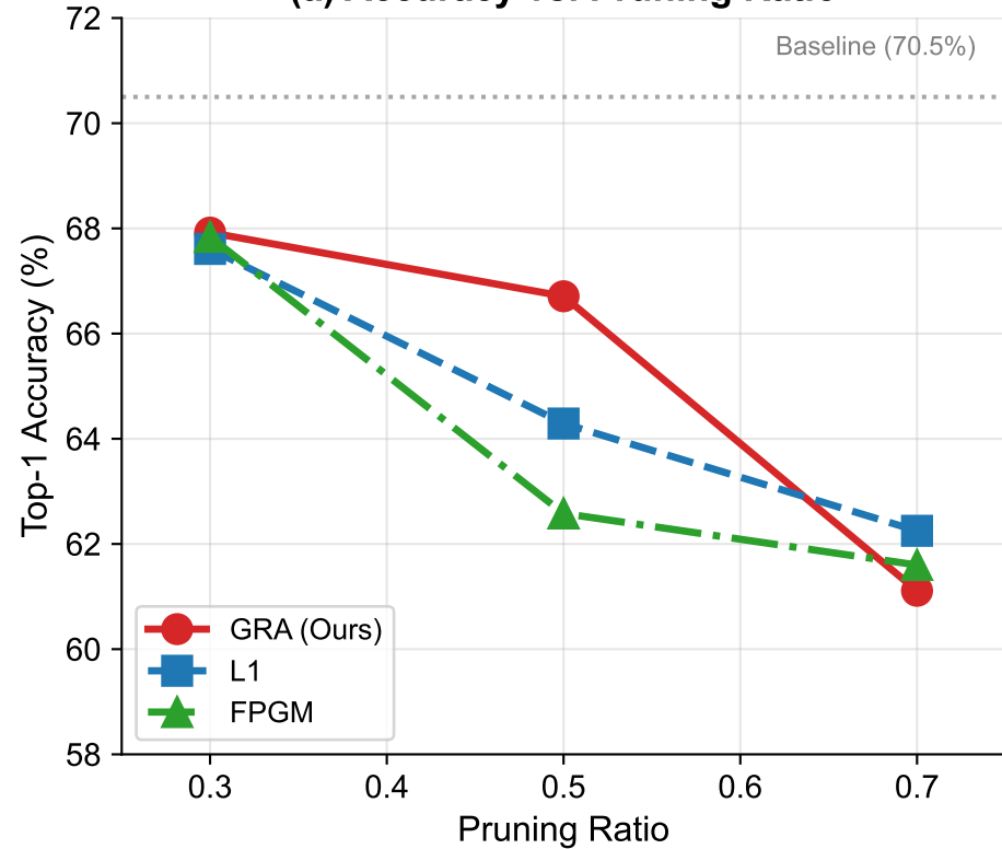
(a) Accuracy vs. Pruning Ratio
