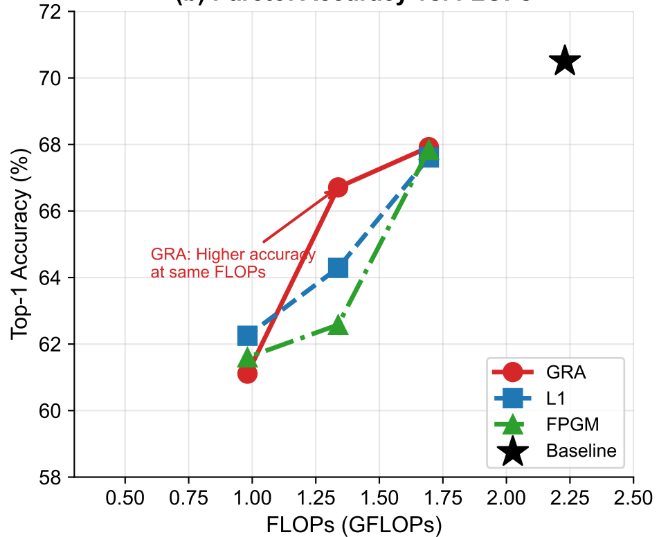
(b) Pareto: Accuracy vs. FLOPs
