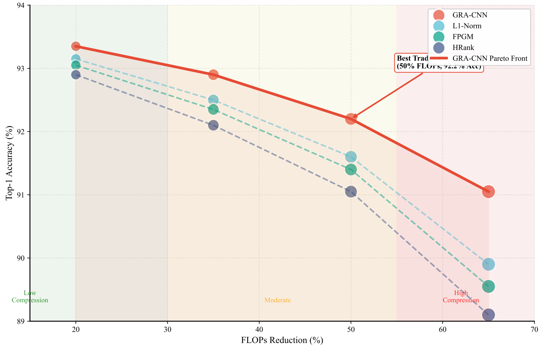
Accuracy-Efficiency Trade-off: ResNet-56 on CIFAR-10 (Bubble size represents model complexity)
