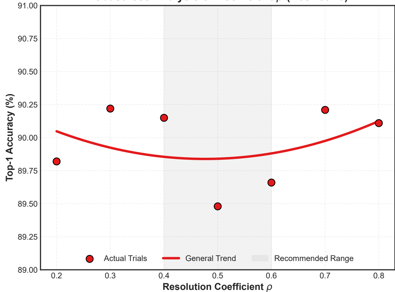
Robustness Analysis of Coefficient \rho (ResNet-20)
