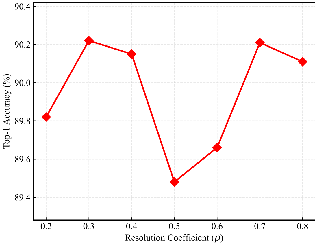
Sensitivity of \rho (ResNet-20)
