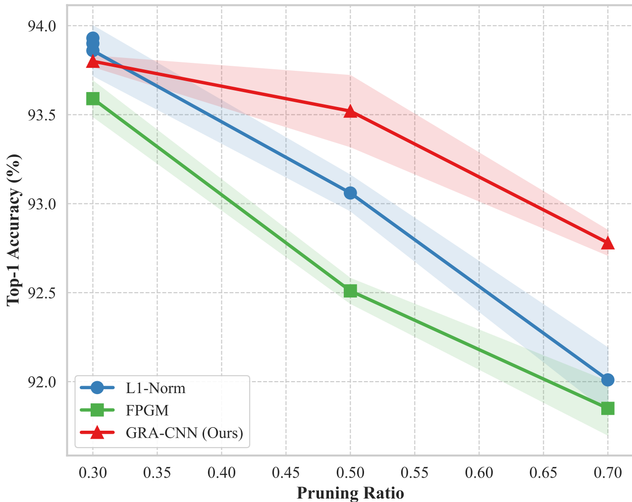
ResNet-110 on CIFAR-10
