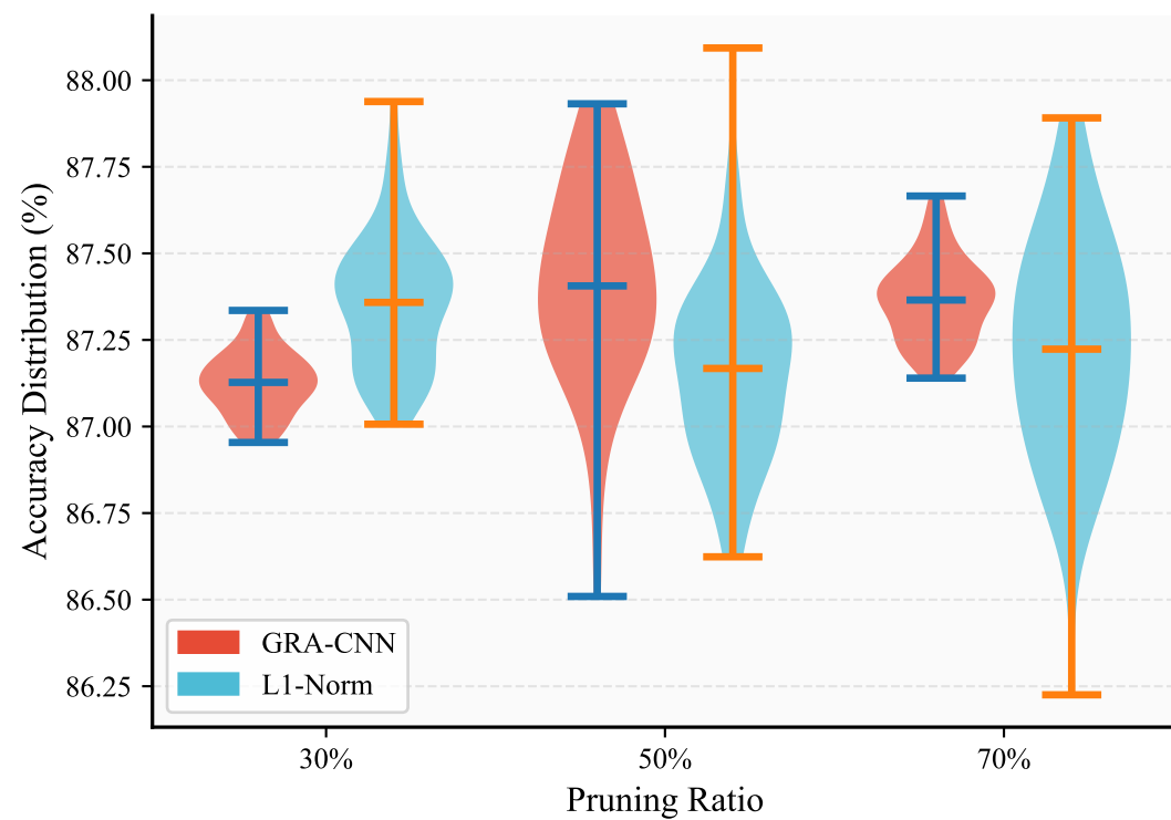
(c) Result Stability (Violin Plot)
