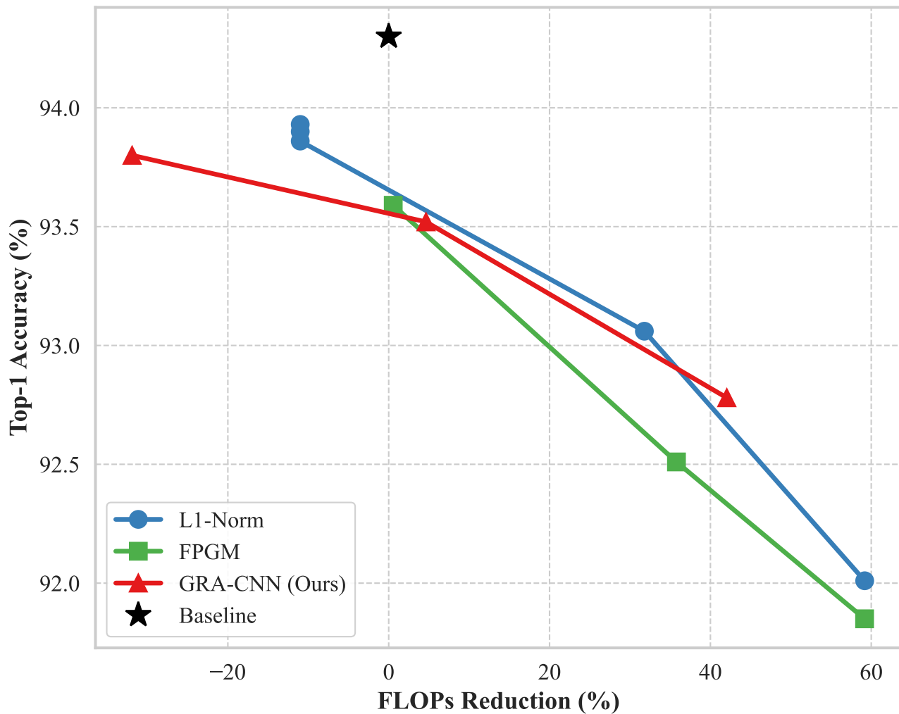
ResNet-110 Efficiency Trade-off
