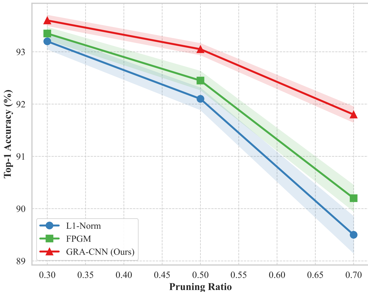
VGG-16 on CIFAR-10
