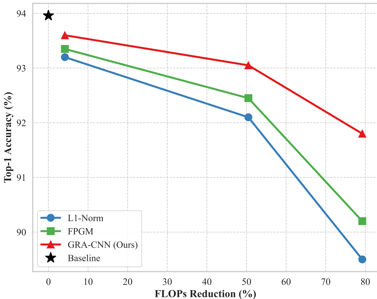
VGG-16 Efficiency Trade-off
