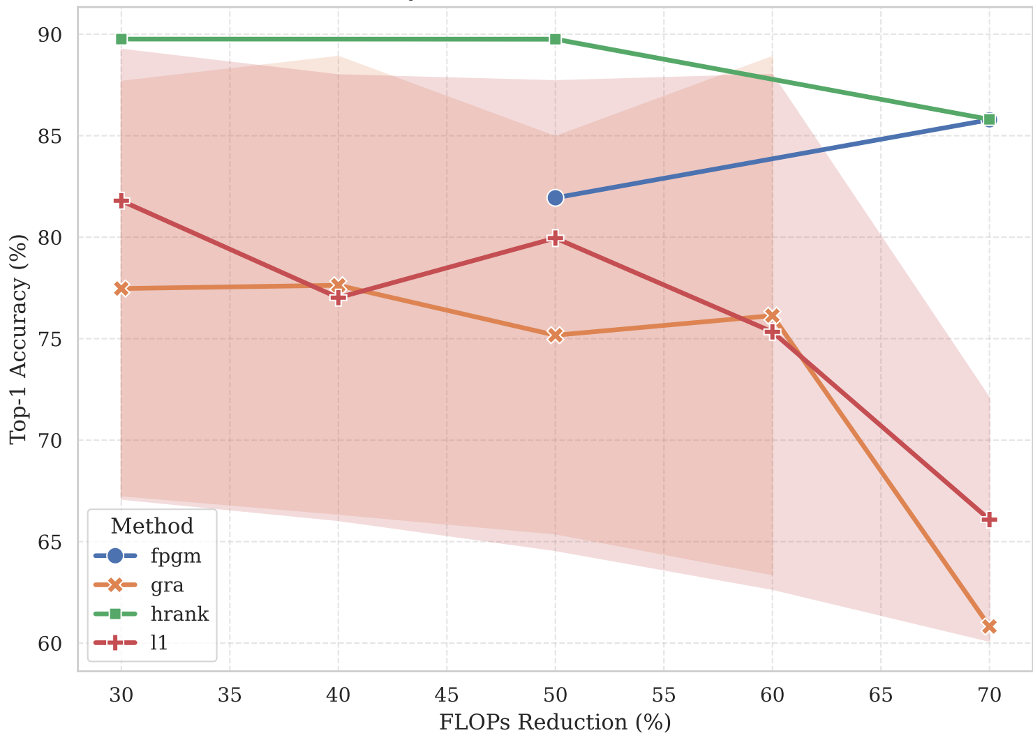
Accuracy vs. FLOPs Reduction (ResNet-20)
