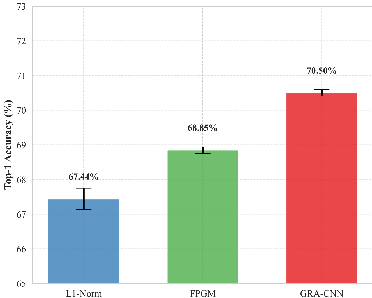
ResNet-56 on CIFAR-100 (Ratio=0.5)
