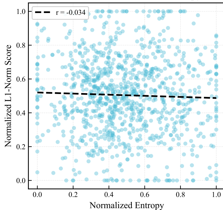
(b) L1-Norm vs Activation Entropy
