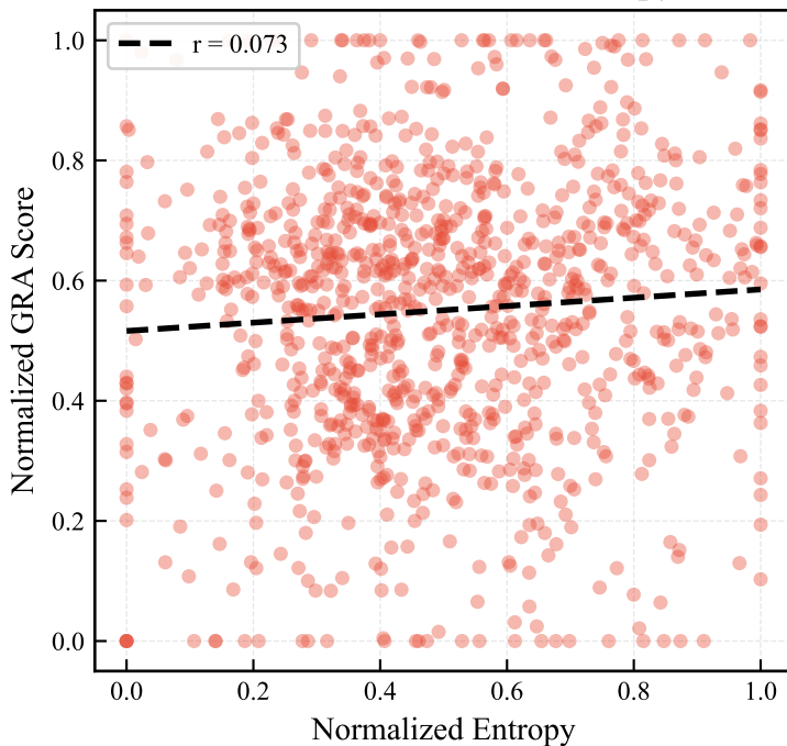
(a) GRA vs Activation Entropy
