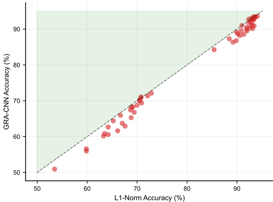
(a) GRA-CNN vs L1-Norm
