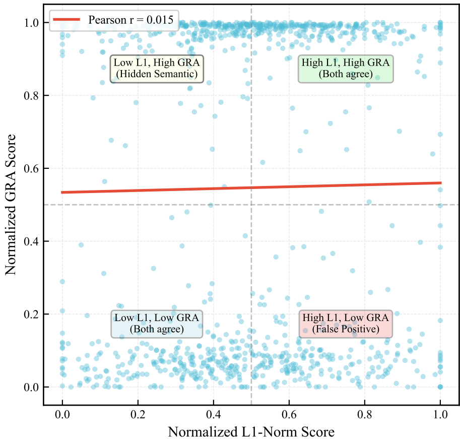
Channel Importance: L1-Norm vs GRA
