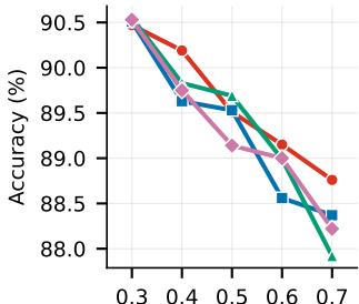
(e) ResNet-20
