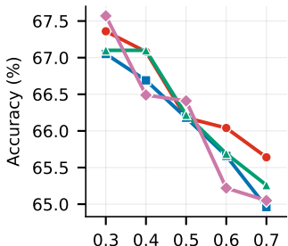
(i) ResNet-20
