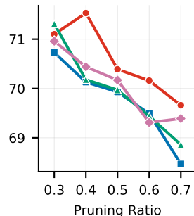
(l) ResNet-56
