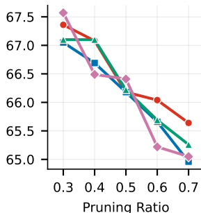
(k) ResNet-20
