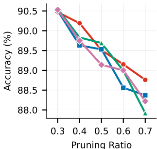
(i) ResNet-20
