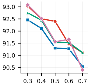
(g) ResNet-110
