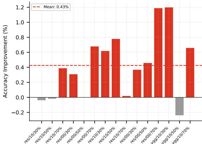
(b) GRA Improvement over L1
