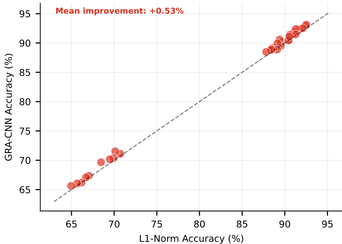
(a) GRA-CNN vs L1-Norm
