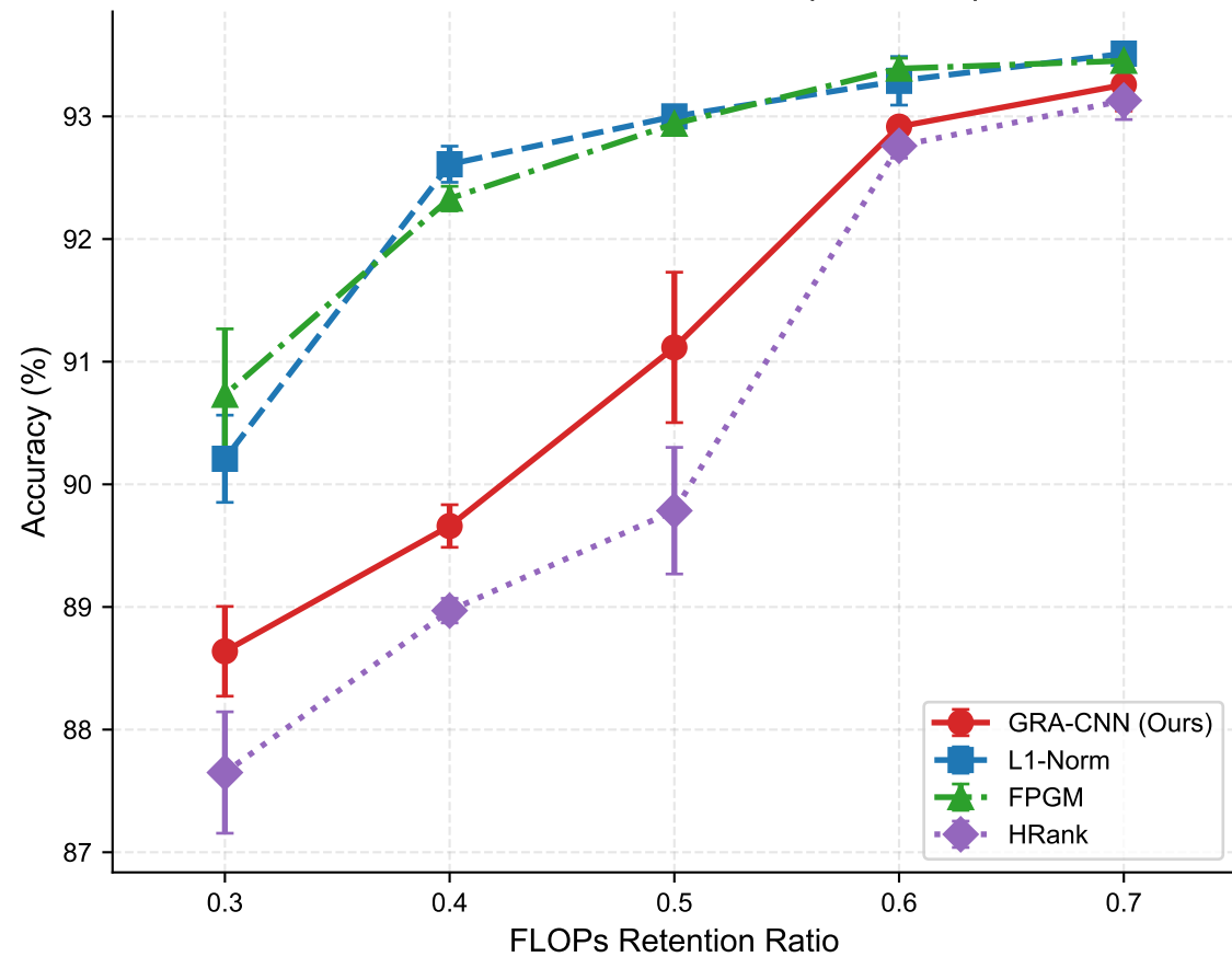
Pareto Frontier on CIFAR-10 (ResNet-56)
