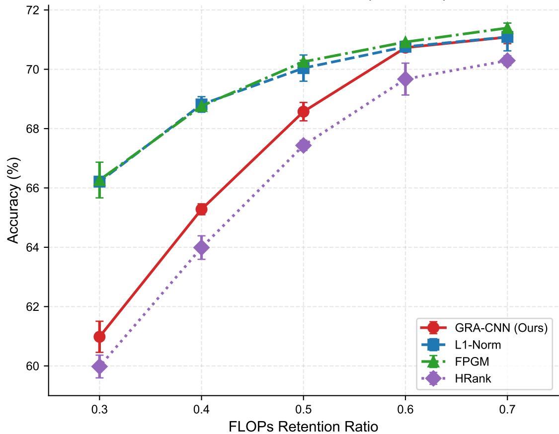
Pareto Frontier on CIFAR-100 (ResNet-56)
