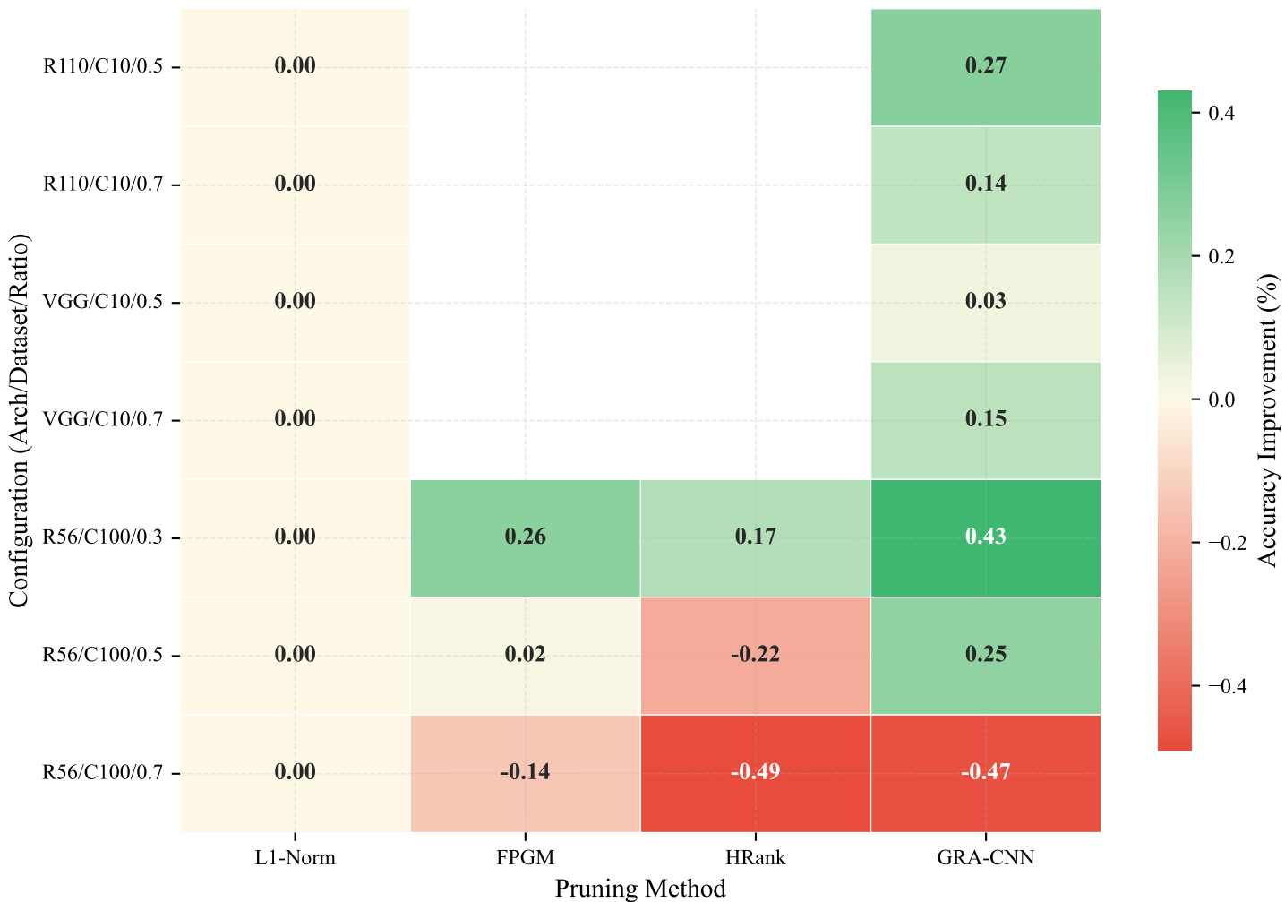
Performance Improvement Heatmap (Relative to L1-Norm Baseline)
