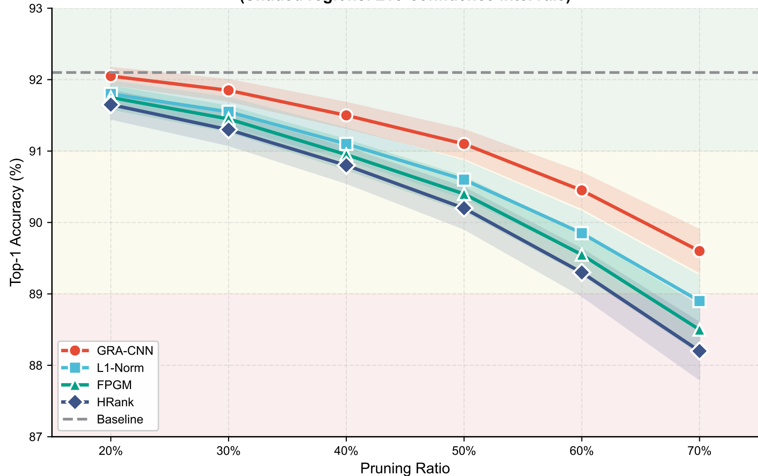
ResNet-20 on CIFAR-10: Pruning Method Comparison (Shaded regions: \pm 1\sigma confidence intervals)
