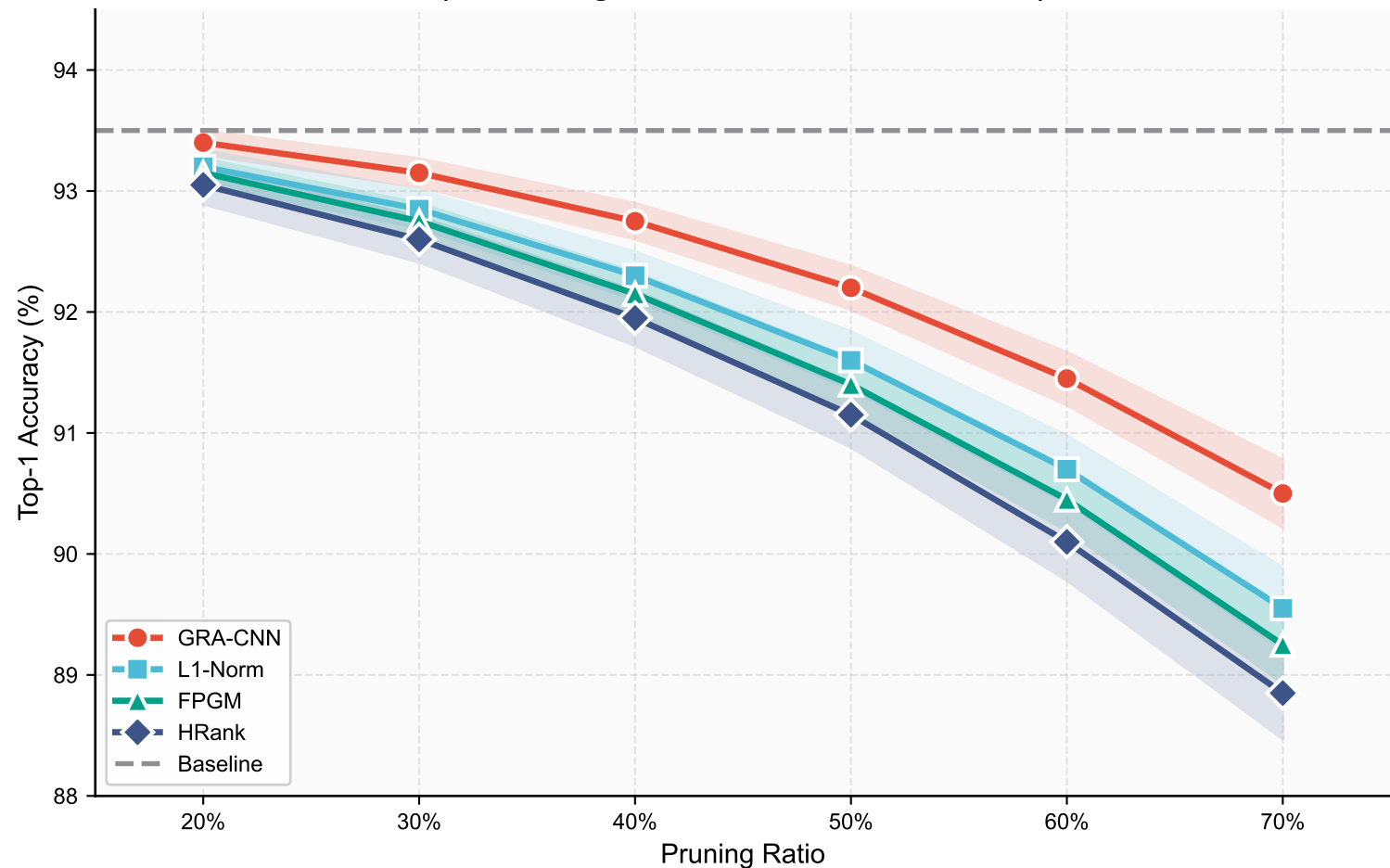
ResNet-56 on CIFAR-10: Pruning Method Comparison (Shaded regions: \pm 1\sigma confidence intervals)
