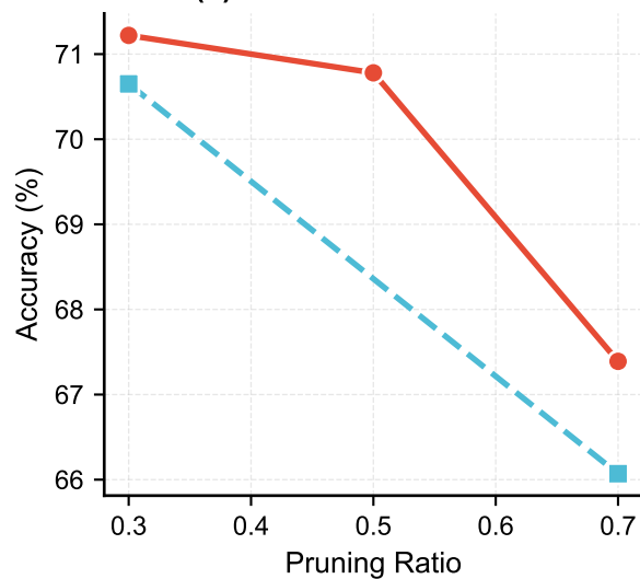
(e) resnet56 on cifar100
