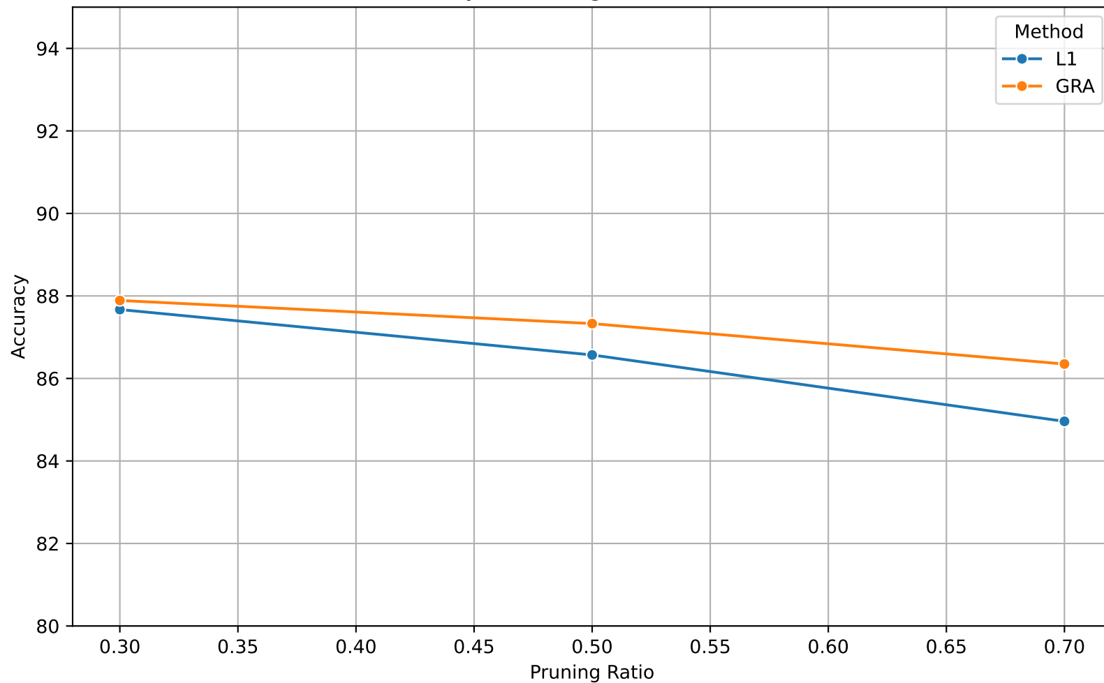
Accuracy vs Pruning Ratio (ResNet-20)
