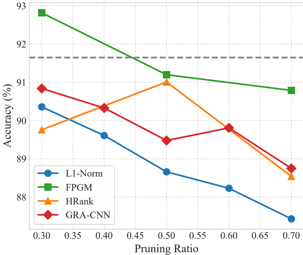
ResNet-20 on CIFAR-10
