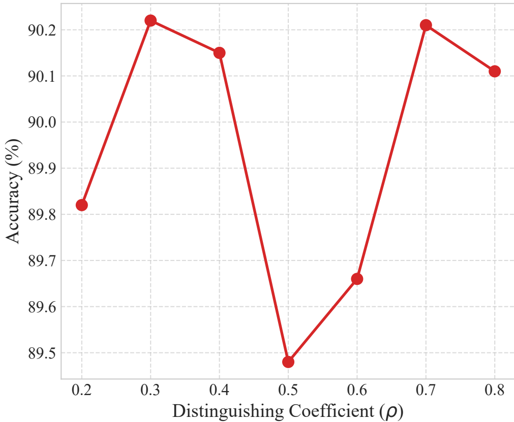
Sensitivity to \rho (ResNet-20, Ratio 0.5)
