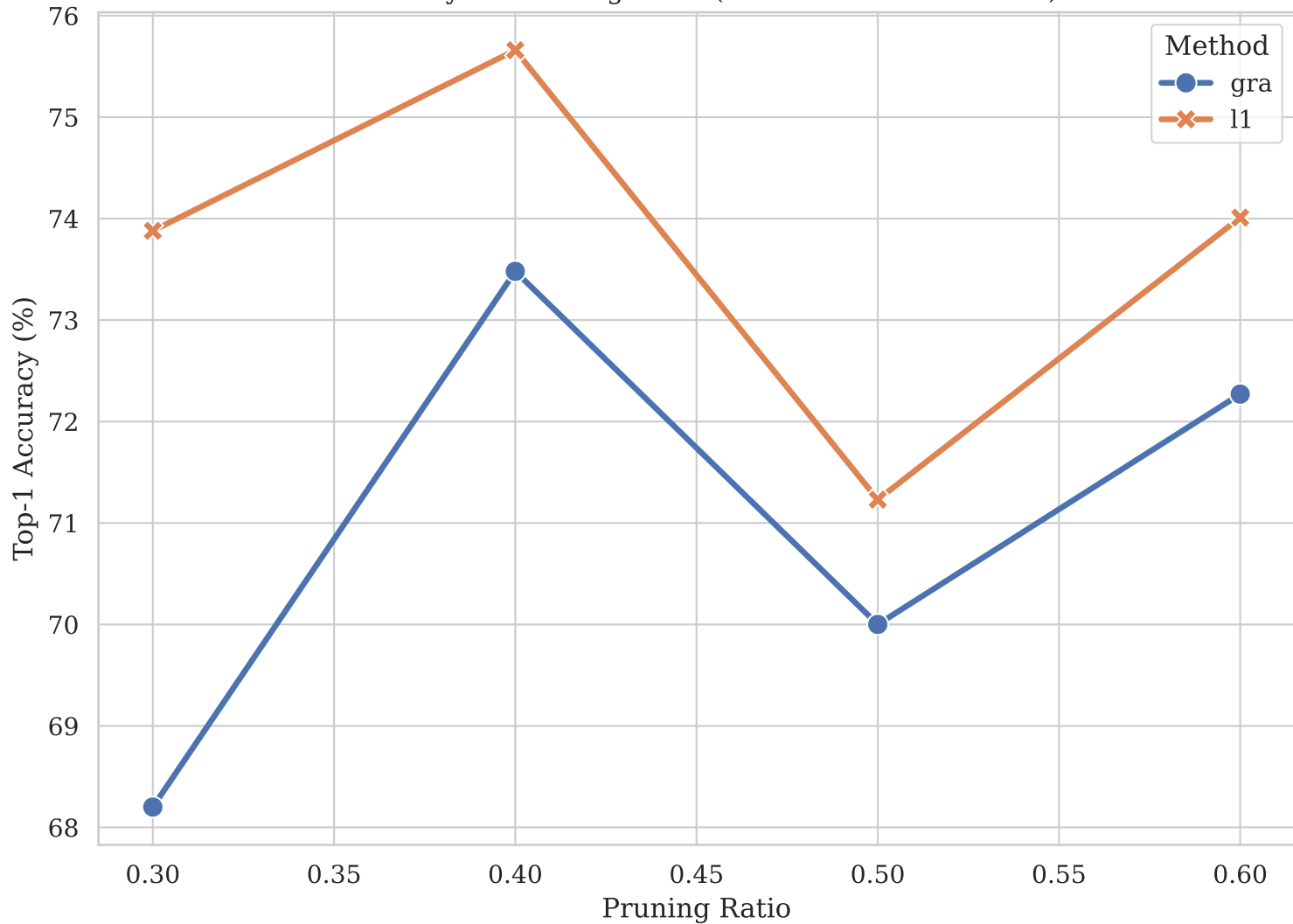
Accuracy vs. Pruning Ratio (ResNet-20 on CIFAR-10)
